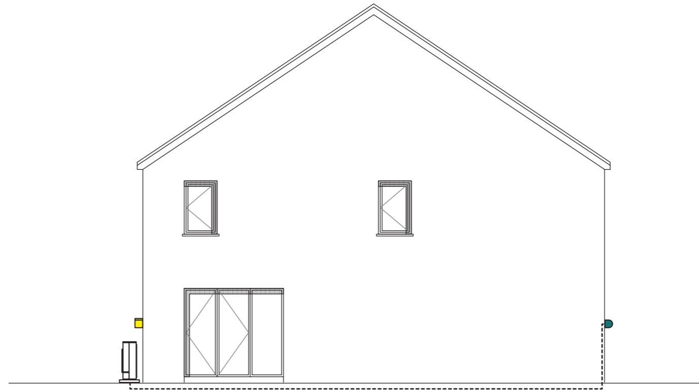
Side Elevation 1:100
