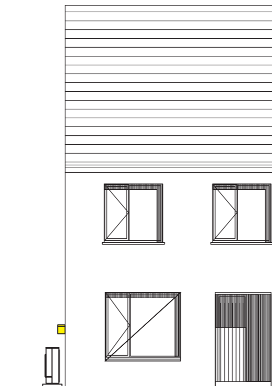
Front Elevation 1:100
