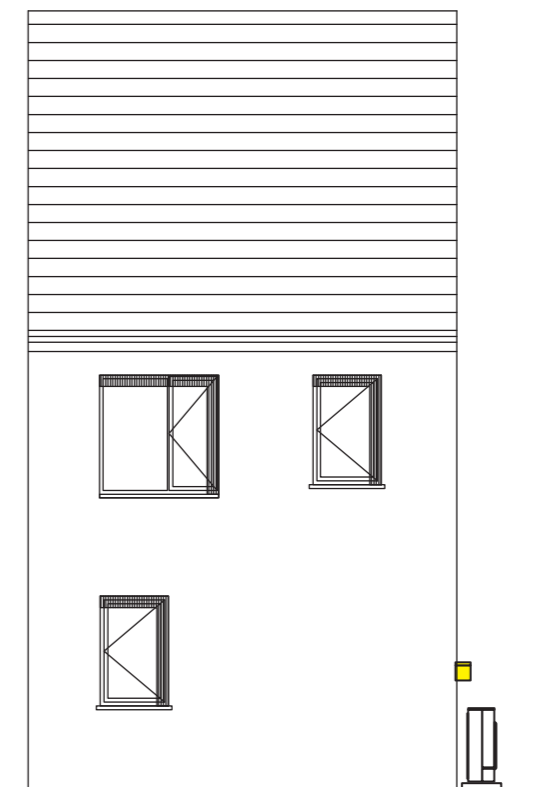
Rear Elevation 1:100
